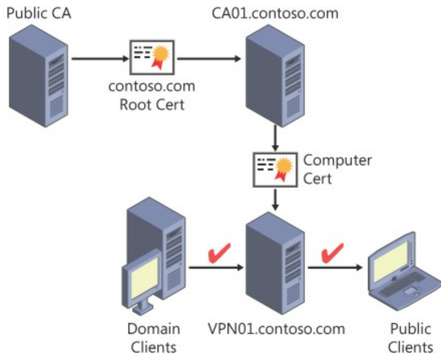
FIGURE 3-1 A hybrid certificate deployment
