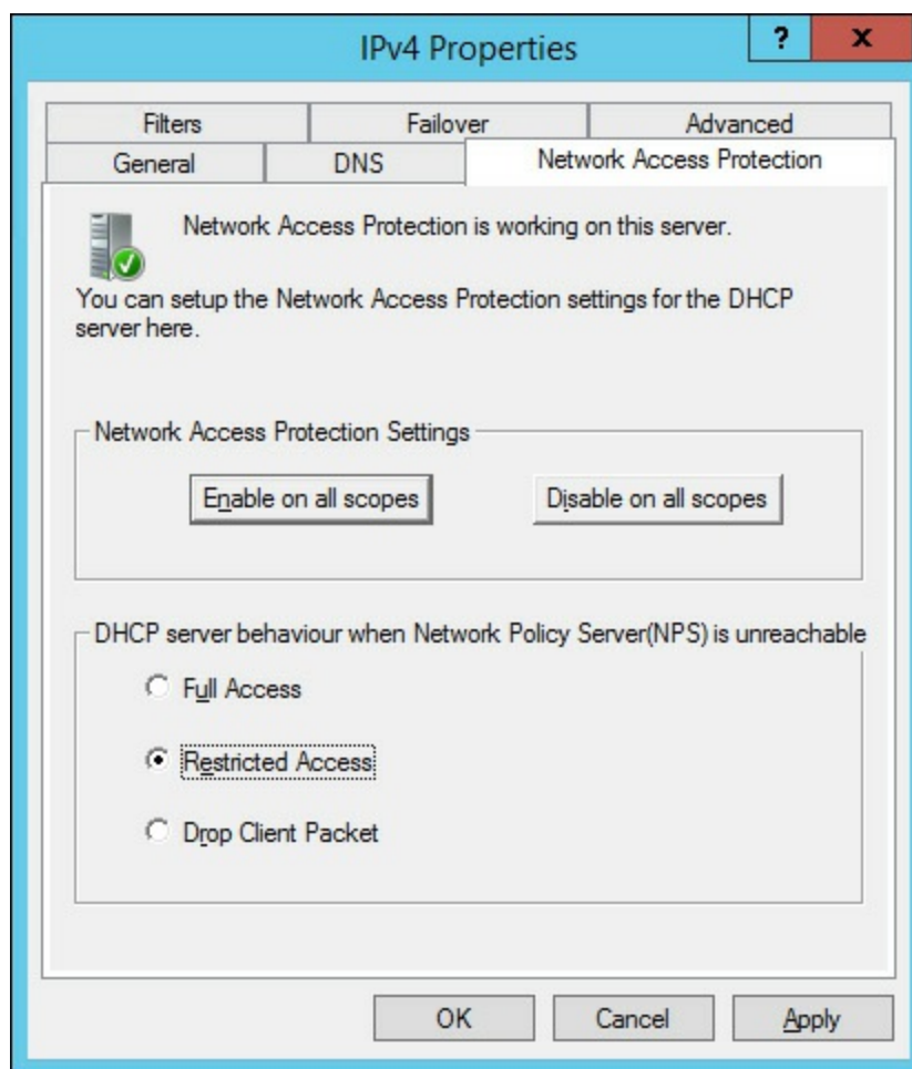
FIGURE 2-7 Enabling NAP enforcement using DHCP
