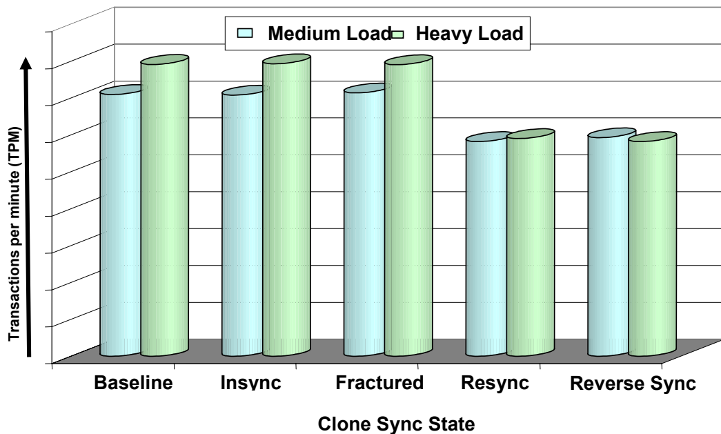
Figure 17. OLTP transactions per minute during various states at a high sync rate—Fibre Channel
