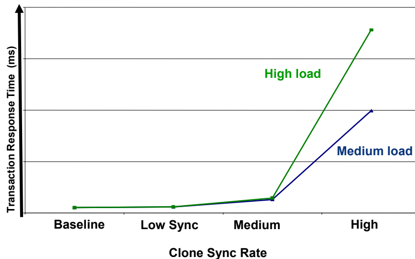
Figure 14. OLTP average response time during initial sync—Fibre Channel
