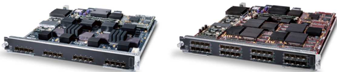
Figure 3. Cisco MDS 9000 Family 16- and 32-Port Fibre Channel Switching Modules
