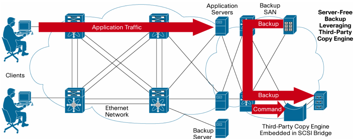
Figure 3. Server-Free Backup Model
