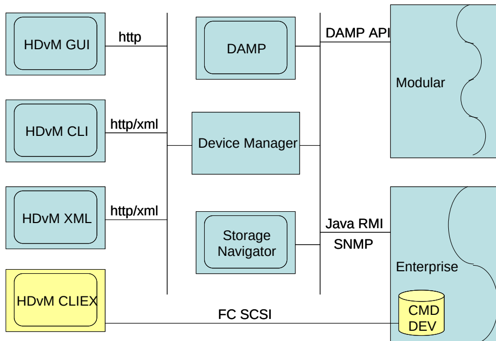
Figure 1-1 Device Manager Communication Protocols
