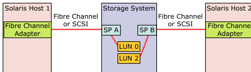
Figure 8-3 Unshared Direct Dual-Server Configuration before Assigning LUN 0
