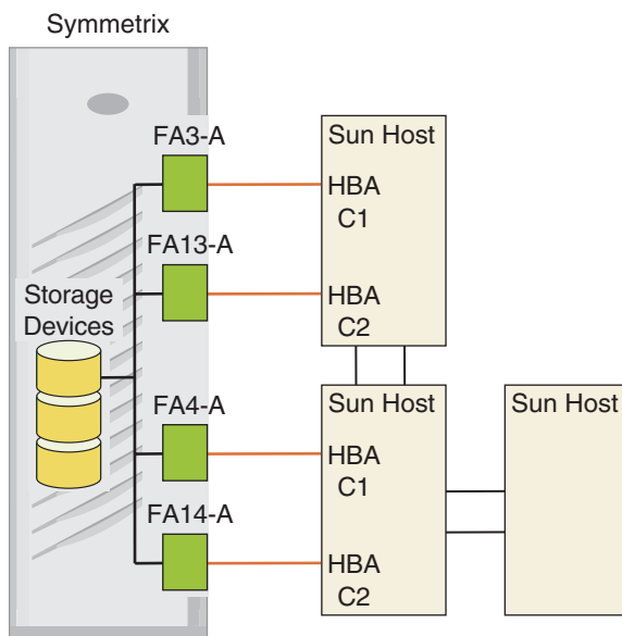
Figure 5-2 Three-Node HA Configuration
