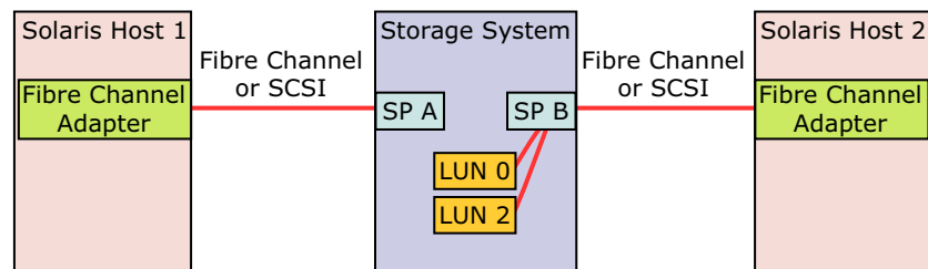
Figure 8-4 Unshared Direct Dual-Server Configuration after Assigning LUN 0
