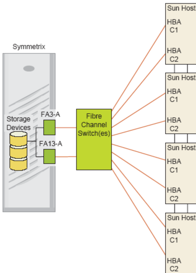
Figure 5-3 Four-Node Fully Attached Configuration
