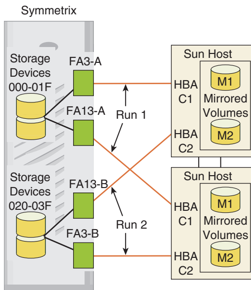
Figure 5-4 Two-Node Host-Based Mirrored Configuration
