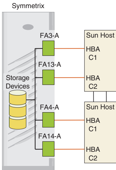
Figure 5-1 Typical Two-Node Topology
