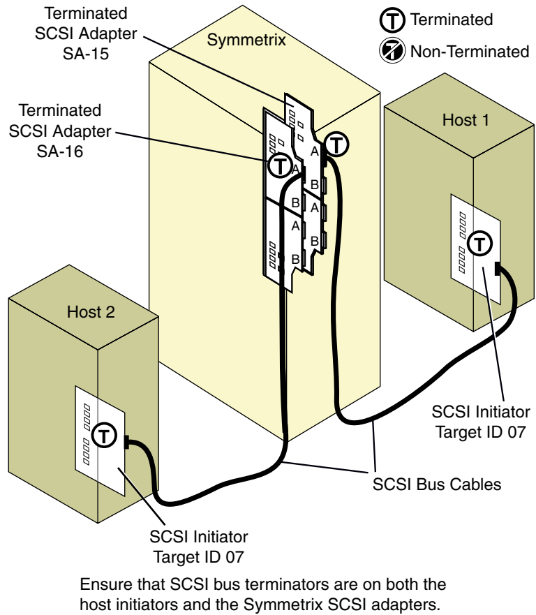
Figure 4-1 Multipath, Single-Initiator, Two-Host Cluster
