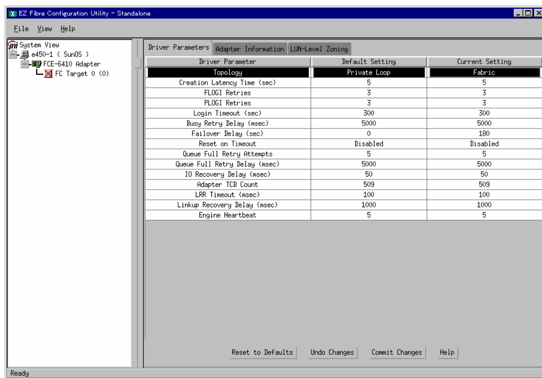
Figure 2.17 Example of JNI™ Driver Parameters for Fabric Switch
