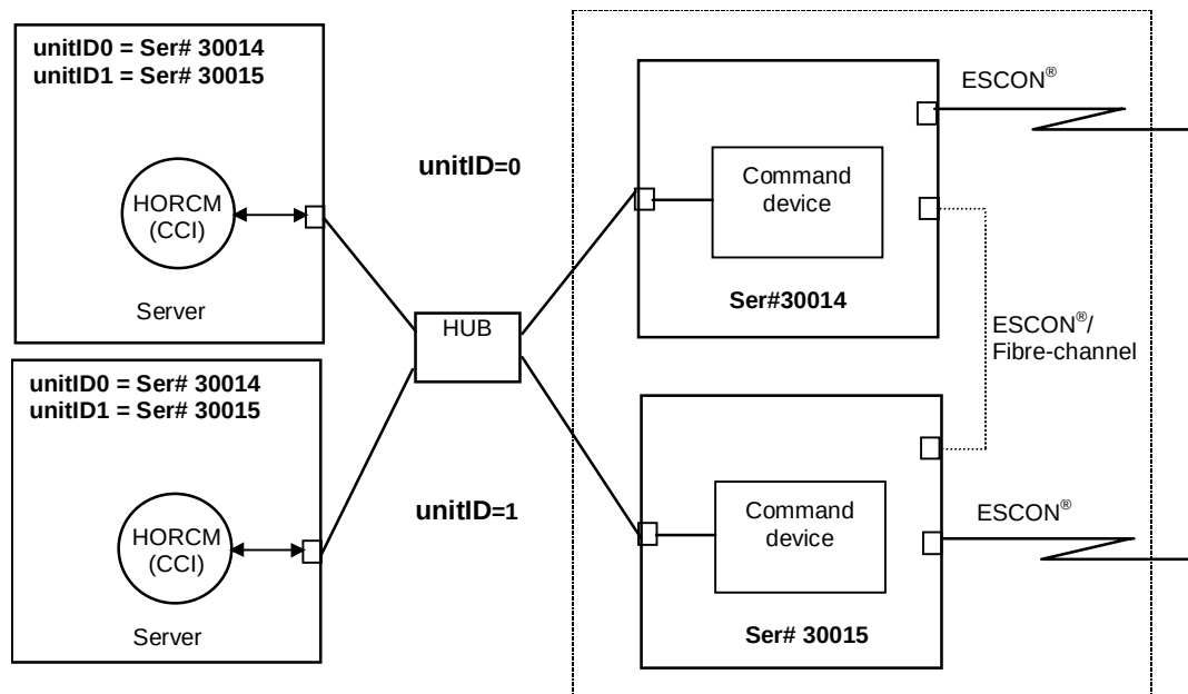
Figure 2.26 Configuration and Unit IDs for Multiple Subsystems
