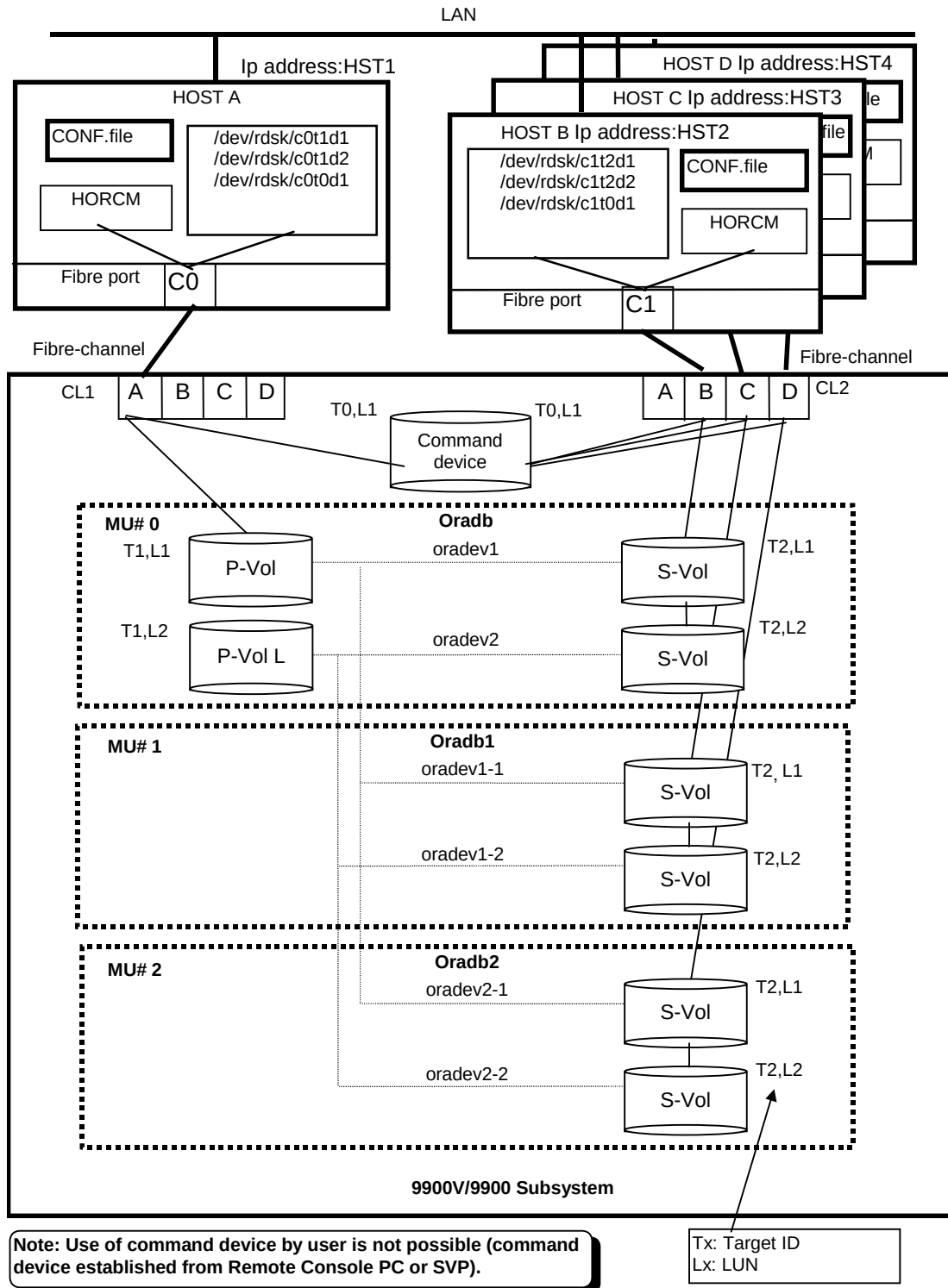
Figure 2.39 ShadowImage Configuration Example (continues on the next page)
