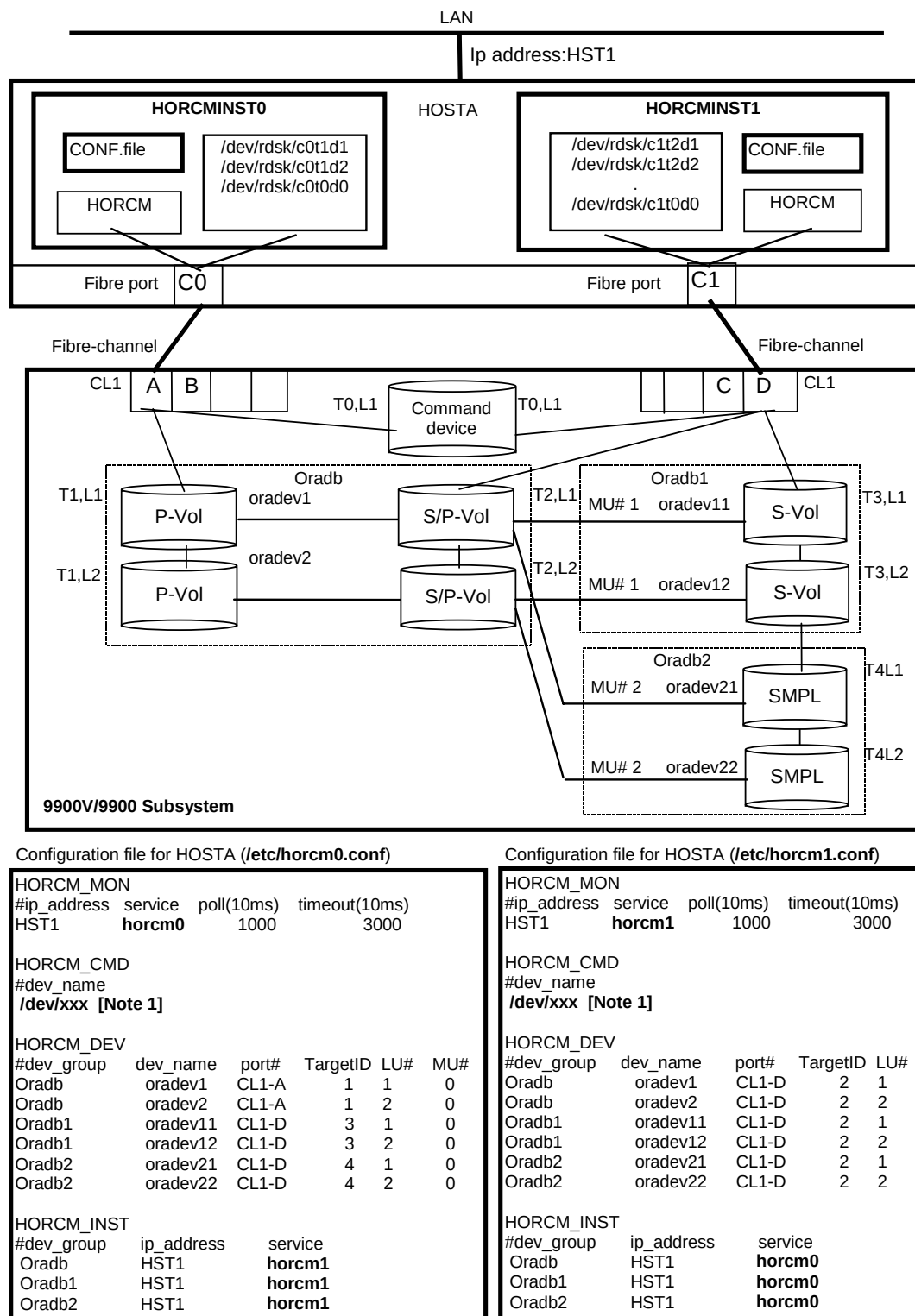
Figure 2.40 ShadowImage Configuration Example with Cascade Pairs
