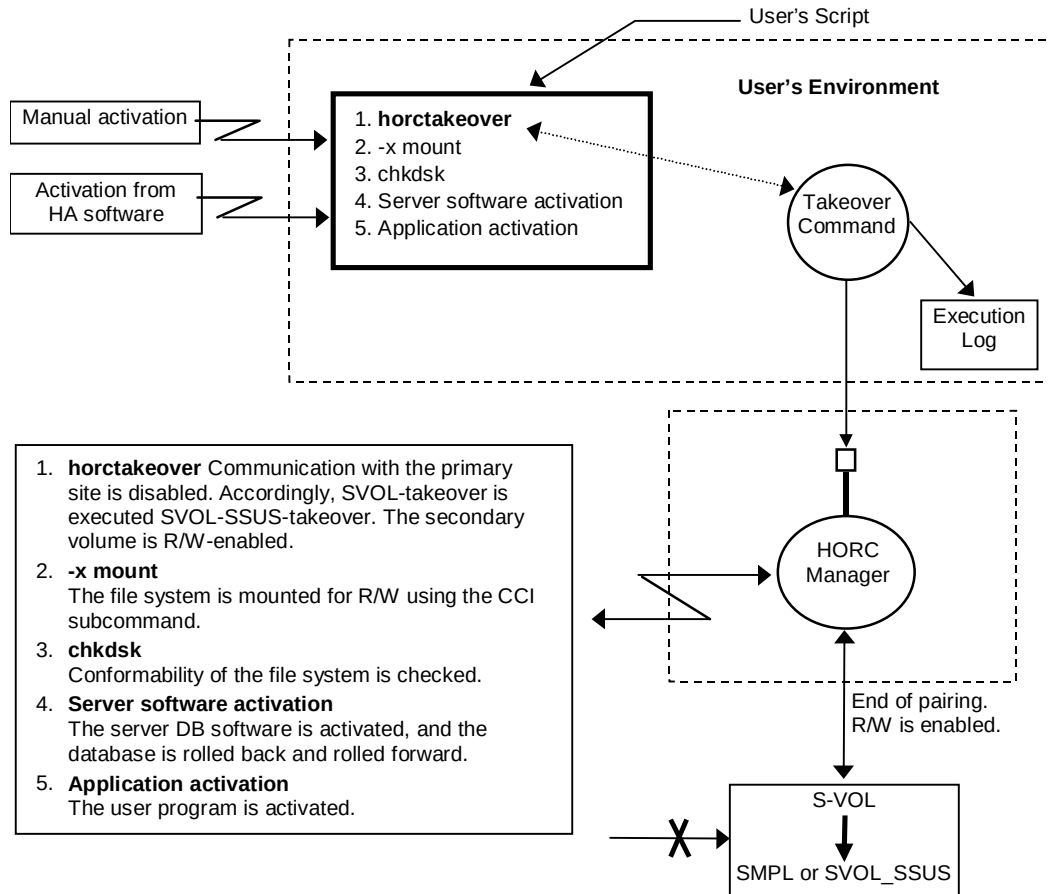
Figure 4.26 Application/Example of Hitachi TrueCopy Takeover (Windows-based System)
