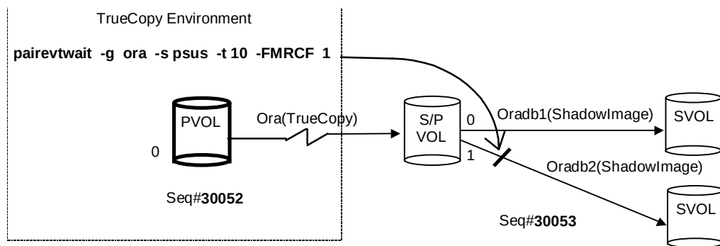
Figure 4.13 Example of -FMRCF Option for Pairevtwait
