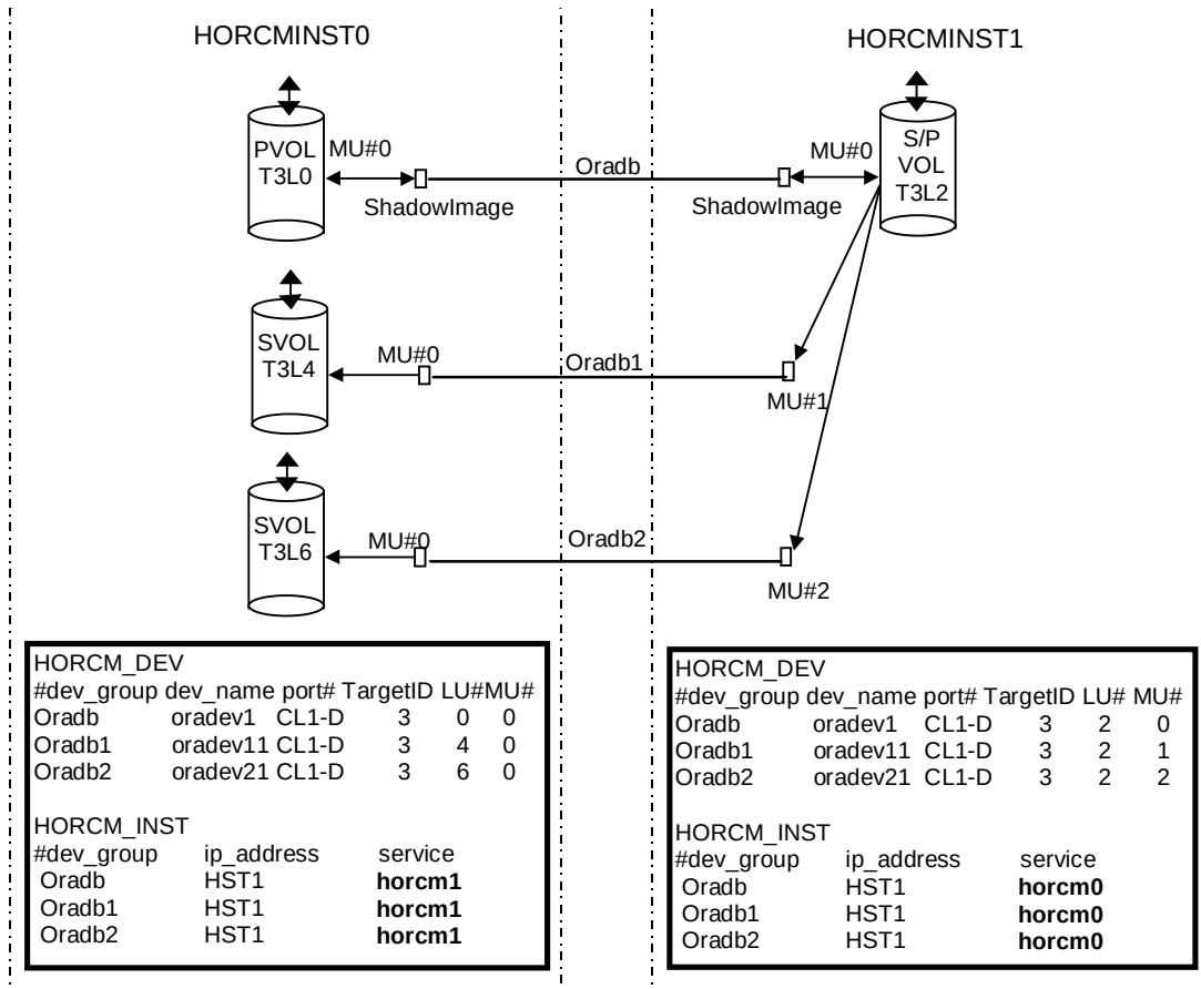
Figure 2.43 ShadowImage Cascade Connection and Configuration File
