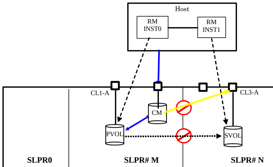
Figure 4.77 SLPR Configuration on a Single Host
