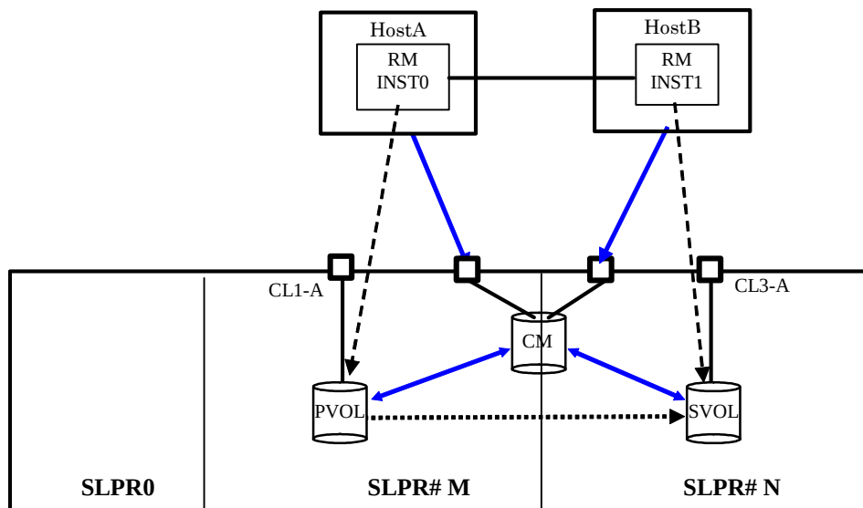
Figure 4.82 Operating SLPR#N by Sharing the Command Device
