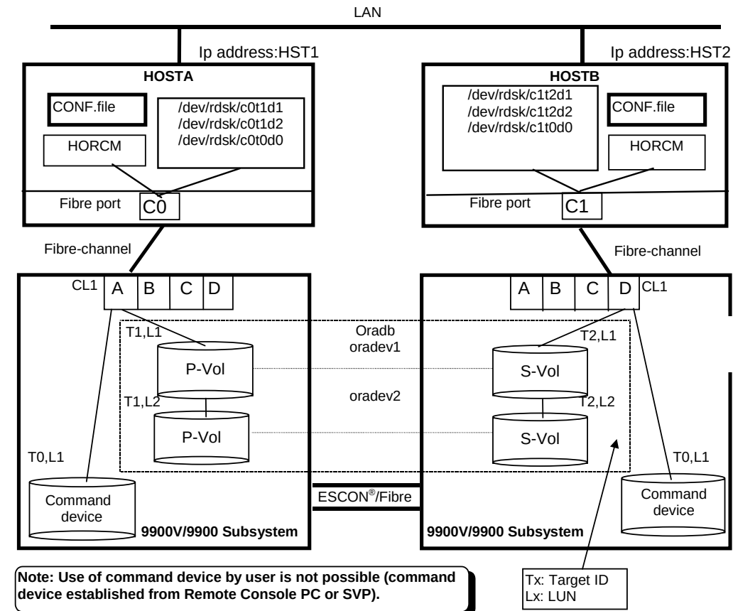
Configuration file for HOSTA (/etc/horcm.conf)
