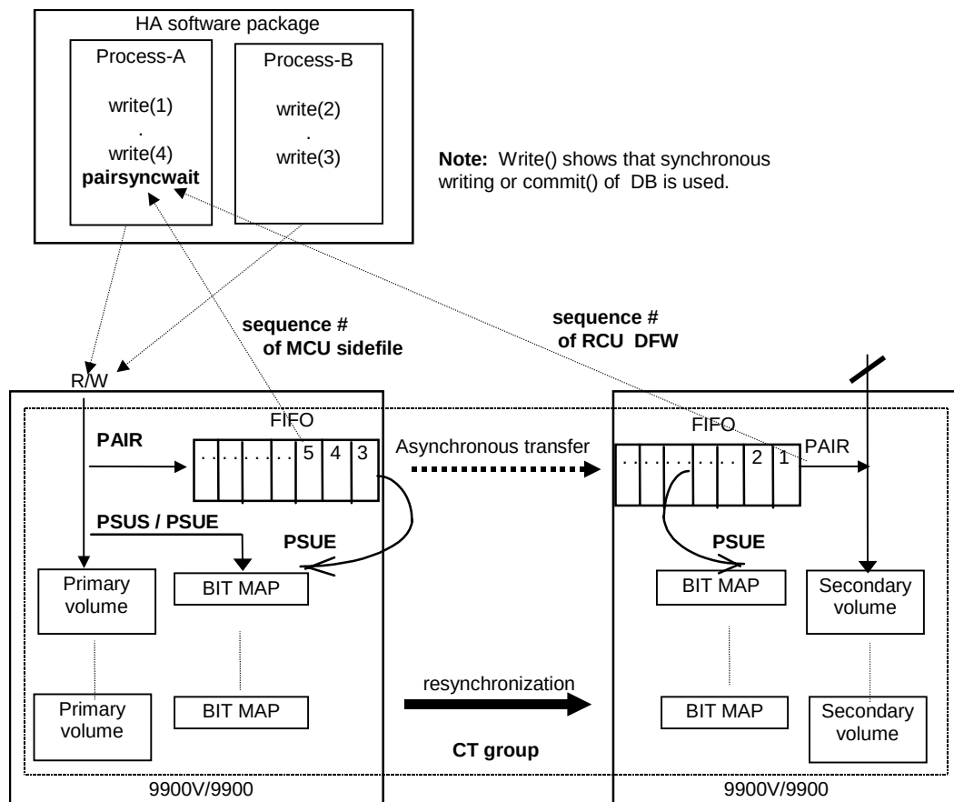
Figure 4.66 Synchronization for Hitachi TrueCopy Async/UR
