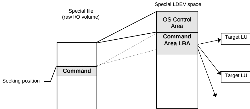
Figure 2.30 Relation between Special File and Special LDEV
