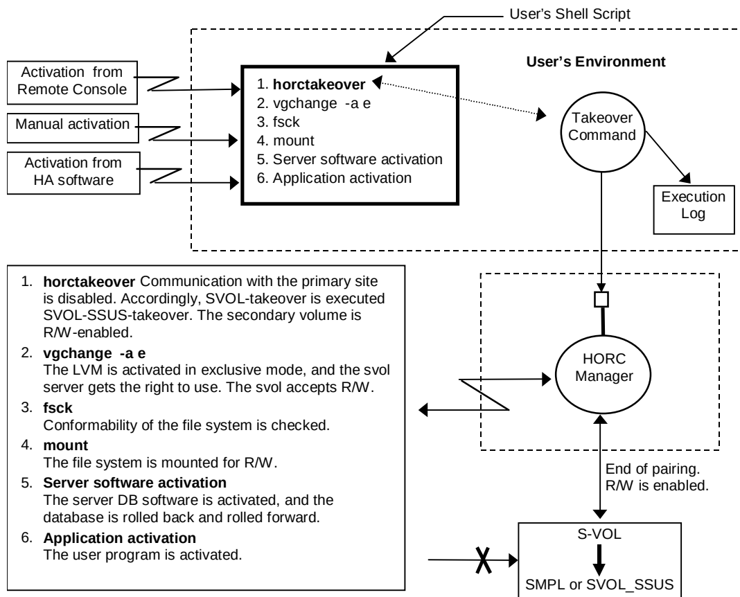
Figure 4.25 Application/Example of Hitachi TrueCopy Takeover (UNIX-based System)
