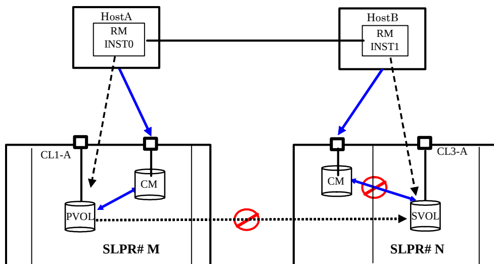
Figure 4.83 TrueCopy Operation using SLPR
