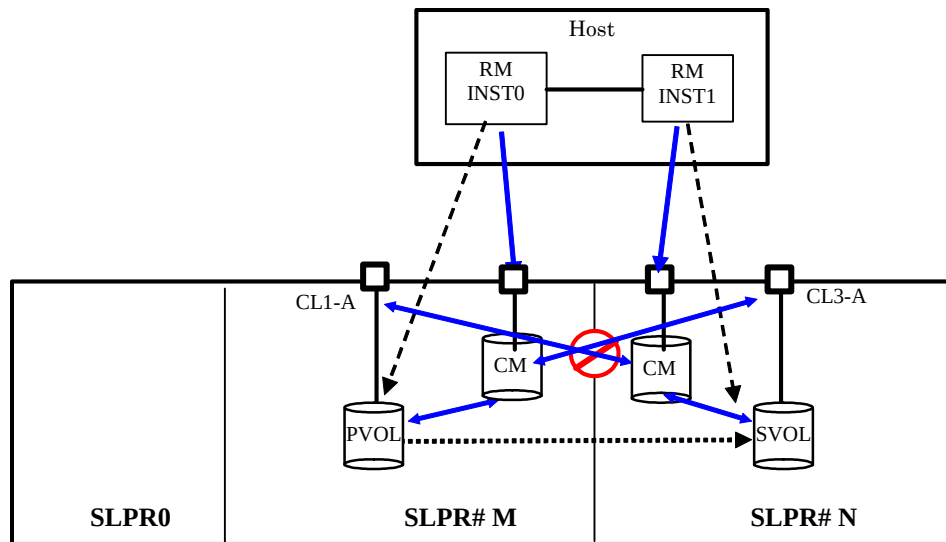
Figure 4.78 Operation Across SLPRs Using two Command Devices on a Single Host
