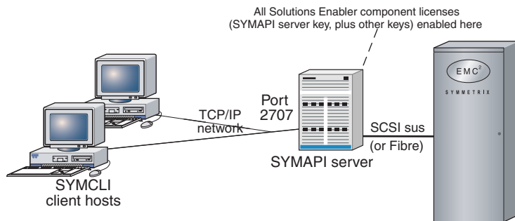
Figure 1 Client/server connection to Symmetrix array
